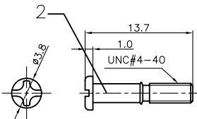
Short BOLT
